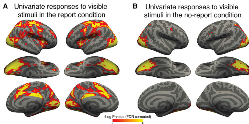
Figure 3. Neural results
