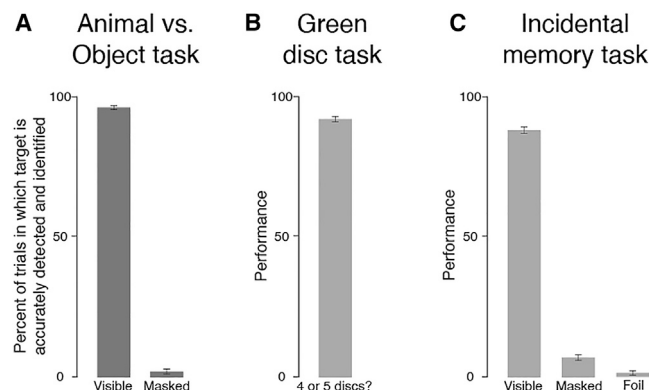
Figure 2. Behavioral results
