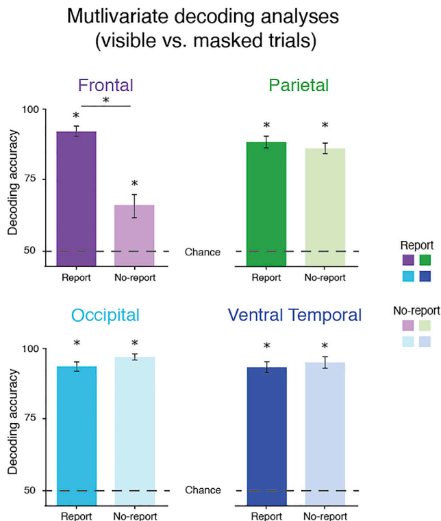
Figure 5. Decoding results
